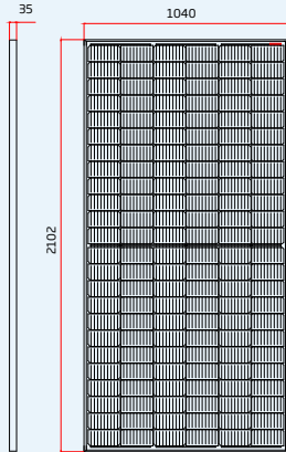
Vista Frontal
